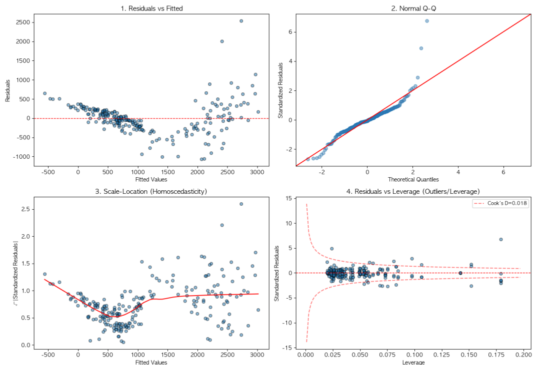
Residual Diagnostics: Four Plots for OLS with Interaction
